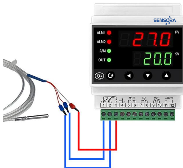
Wiring of PT100 thermocouple
