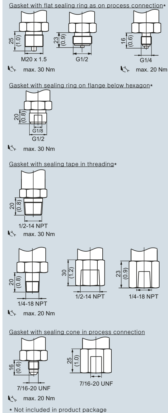
SITRANS P220, process connections, dimensions in mm (inch)
